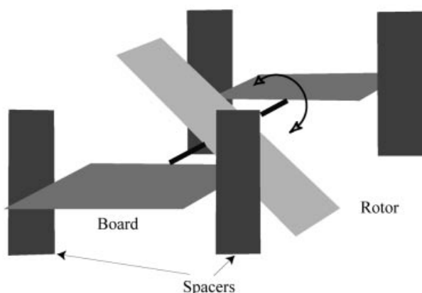
Figure 1. Perspective view of a CPK model of 1 showing the minimum energy conformation under vacuum; the di- tert -butylphenyl spacers' planes are maintained nearly perpendicular to the main board plane by steric crowding
