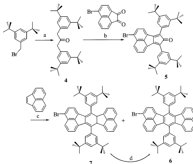
Scheme 3. Synthesis of the main board: (a) TosMIC, NaH, DMF; HCl, CH 2 Cl 2 , 45%; (b) KOH, MeOH, 92%; (c) o -xylene or toluene; (d) DDQ, CH 2 Cl 2
