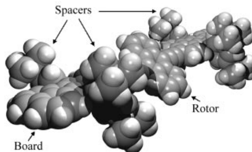
Scheme 1. General scheme of a lander with rotor
