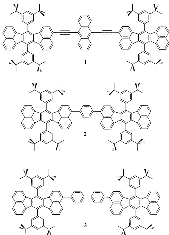
Scheme 2. Landers with a rotor
