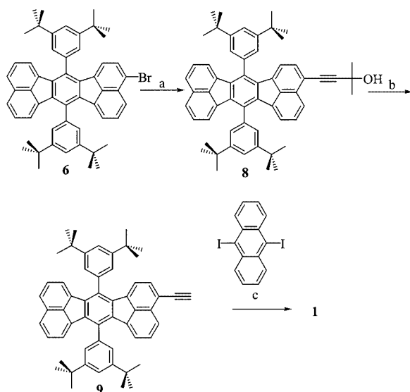
Scheme 4. Synthesis of compound 1 : (a) 2-methyl-3-butyn-2-ol, Pd(PPh 3 ) 4 , PPh 3 , CuI, LiBr, piperidine, 91%; (b) t BuOK, THF, 92%; (c) Pd(PPh 3 ) 2 Cl 2 , CuI, piperidine, THF, 61%
