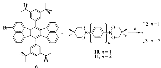
Scheme 5. Synthesis of 2 and 3 : Pd 2 (dba) 3 , t Bu 3 P, CsF, THF, 41% ( 2 ), 46% ( 3 )
